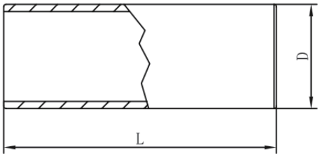
Outline dimensional drawing for 10 x 38, 14 x 51, 22 x 58 copper straight pipes
